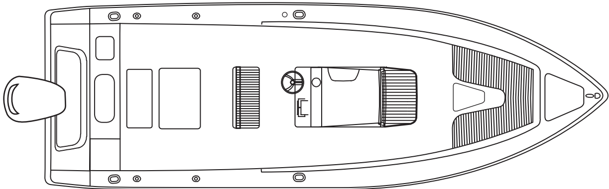
Jupiter 26 Forward Seating with single engine
